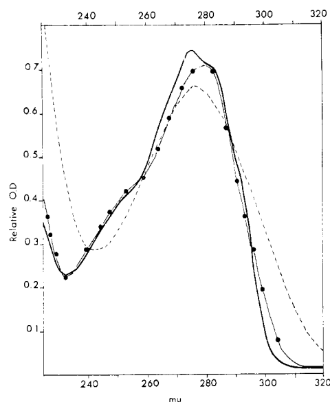
FIGURE 2: The ultraviolet absorption spectra of synthetic N 6 -(threonyl)adenine; pH 1.4, —; pH 7.1, ---; pH 11.6, ····.
