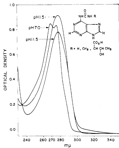
FIGURE 1: The ultraviolet absorption spectra of derivatives of N -(purin-6-yl)urea.
