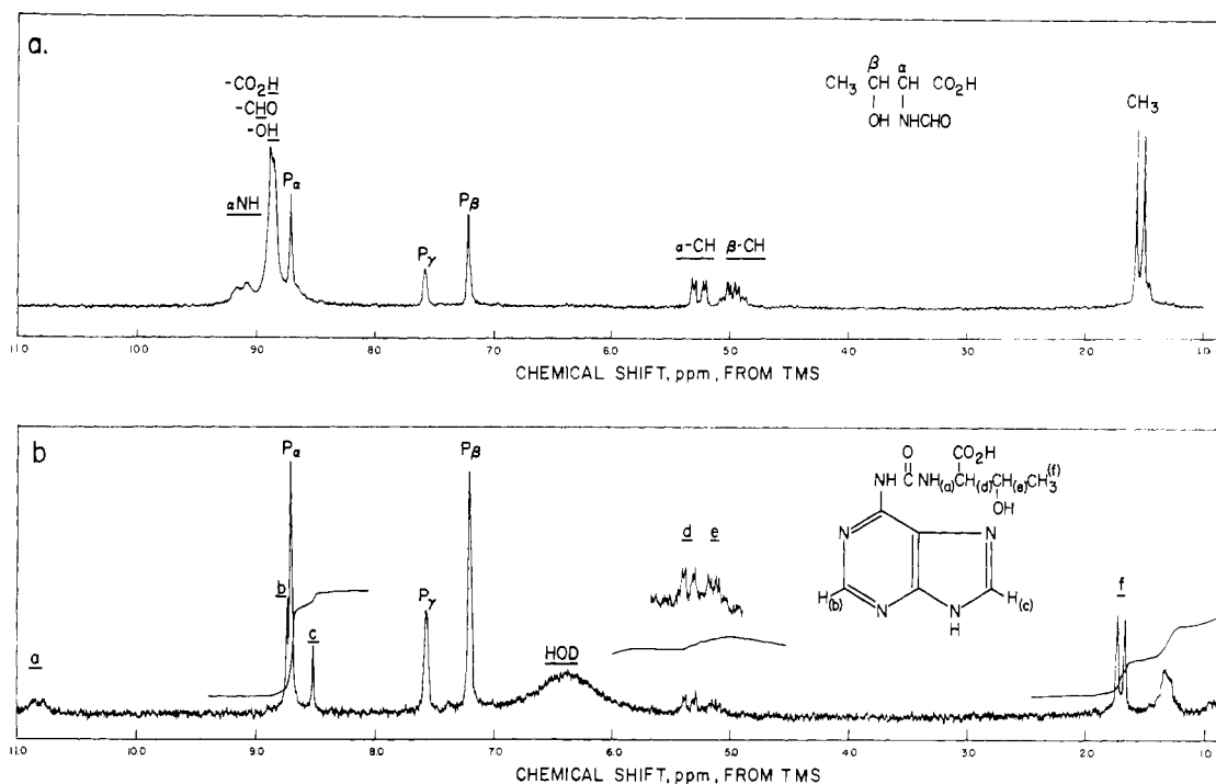
FIGURE 4: Nuclear magnetic resonance spectra taken at 100 MHz; chemical shifts are measured from an internal tetramethylsilane signal. (a) N -Formylthreonine, 0.1 M in pyridine- d_5 . (b) N -(Purin-6-ylcarbamoyl)threonine ( 1 ) 0.04 M in pyridine- d_5 .
