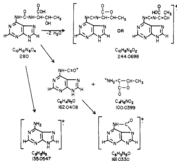
FIGURE 3: The fragmentation pattern of N -(purin-6-ylcarbamoyl)-threonine (1) obtained in the high-resolution mass spectrometer.
